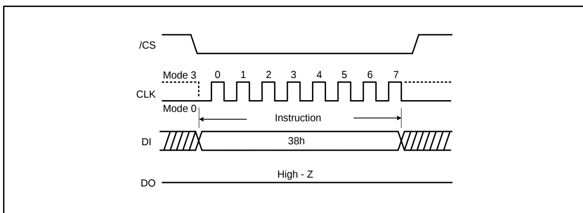
Figure 53. Enter QPI Instruction (SPI Mode only)
