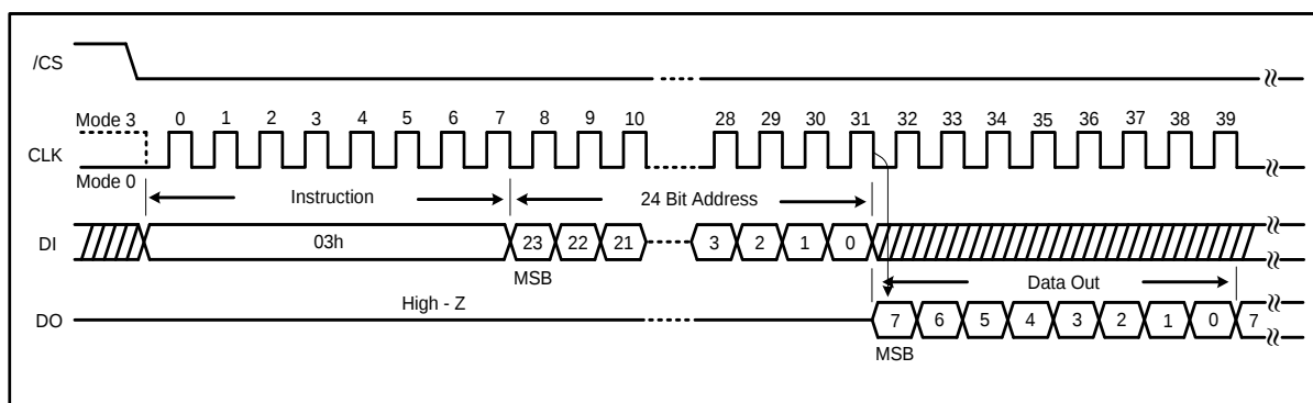
Figure 18. Read Data Instruction (SPI Mode only)
